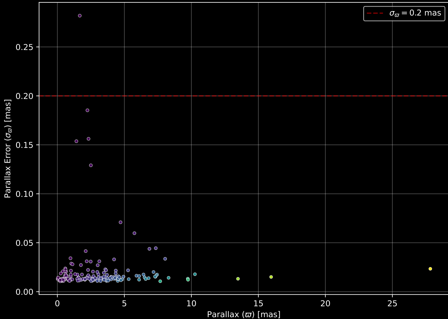
APOGEE DR17 Field: [041+47_MGA] Parallax Quality (n= 169)
