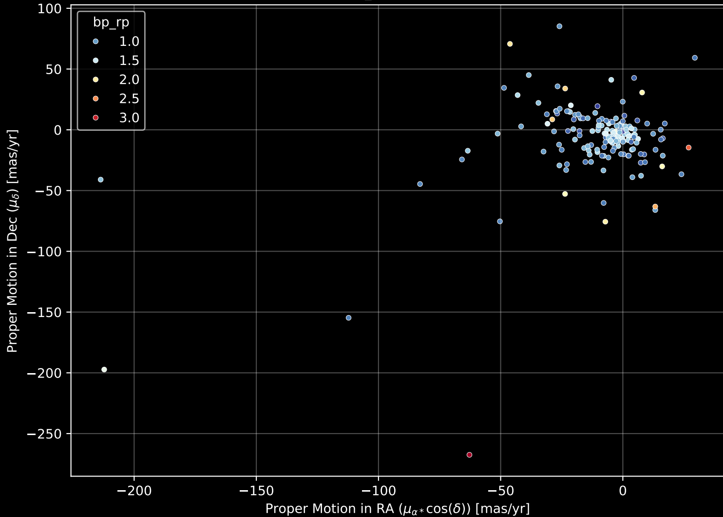
APOGEE DR17 Field: [041+47_MGA] Proper Motion Diagram (n= 169)
