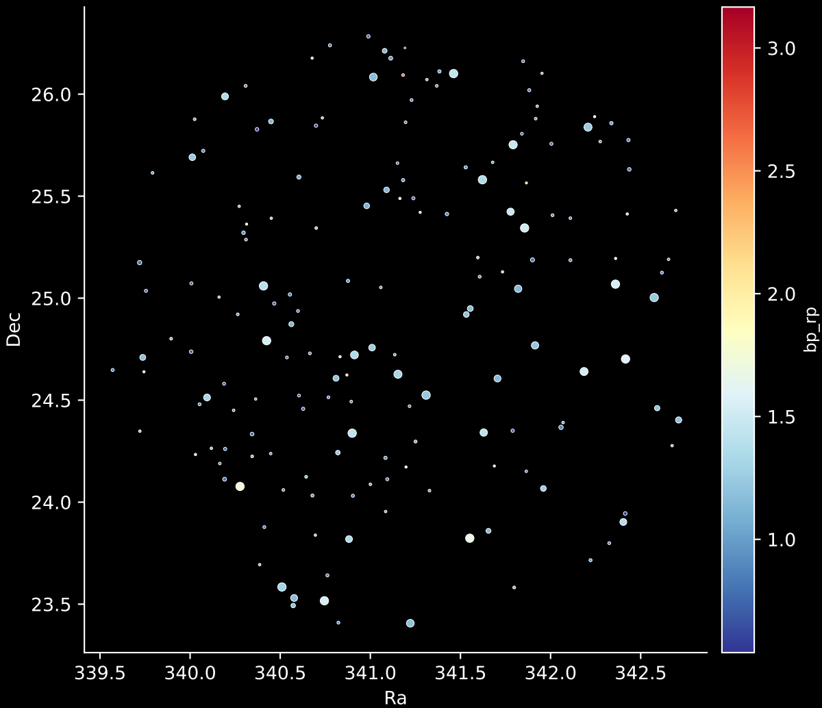
APOGEE DR17 Field: [041+47_MGA] Stars: 169
