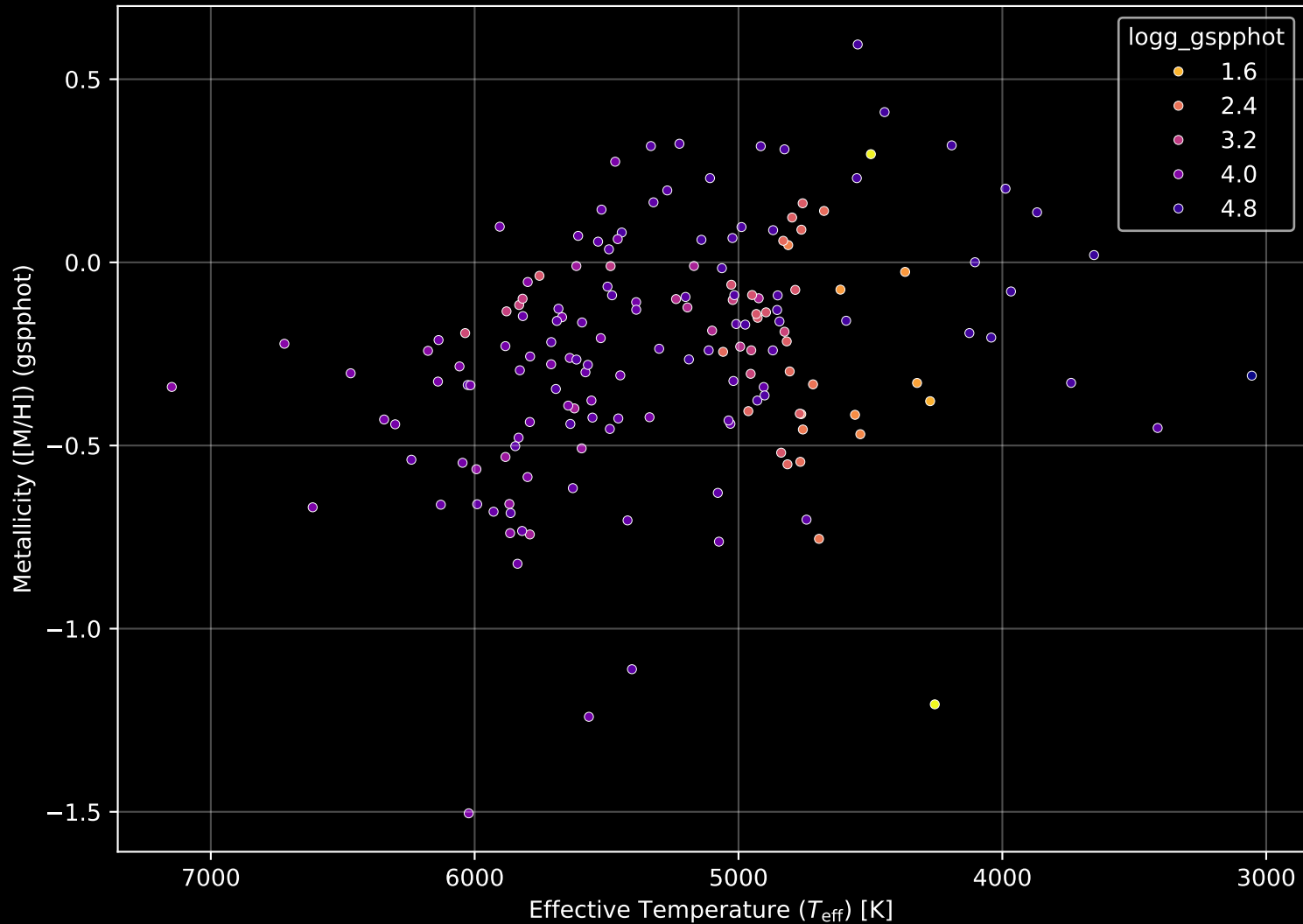
APOGEE DR17 Field: [041+47_MGA] Stellar Population Parameters (n= 169)
