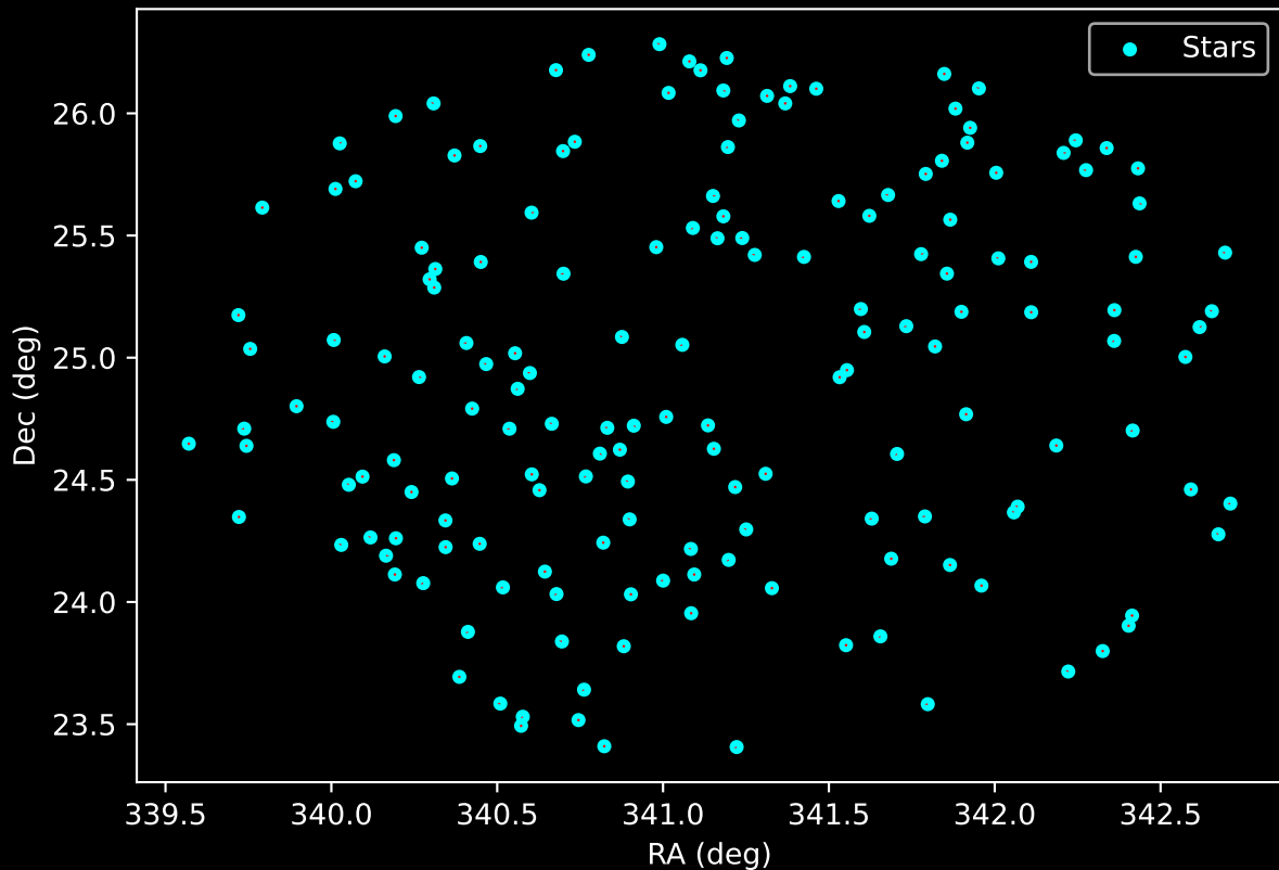
APOGEE DR17 Field: [041+47_MGA] Proper Motion Vectors for Gaia Star Field (n= 169)
