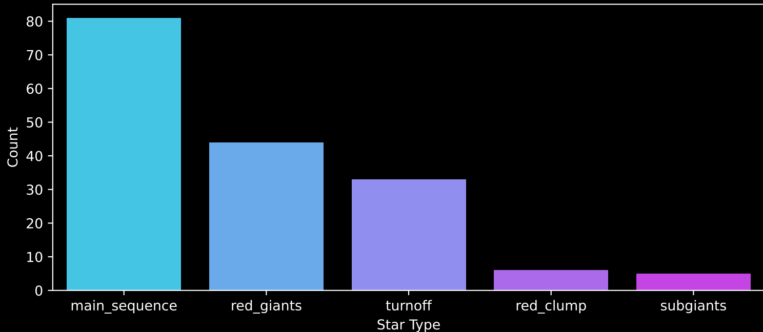
APOGEE DR17 Field: [041+47_MGA] Count plot of Star Type
