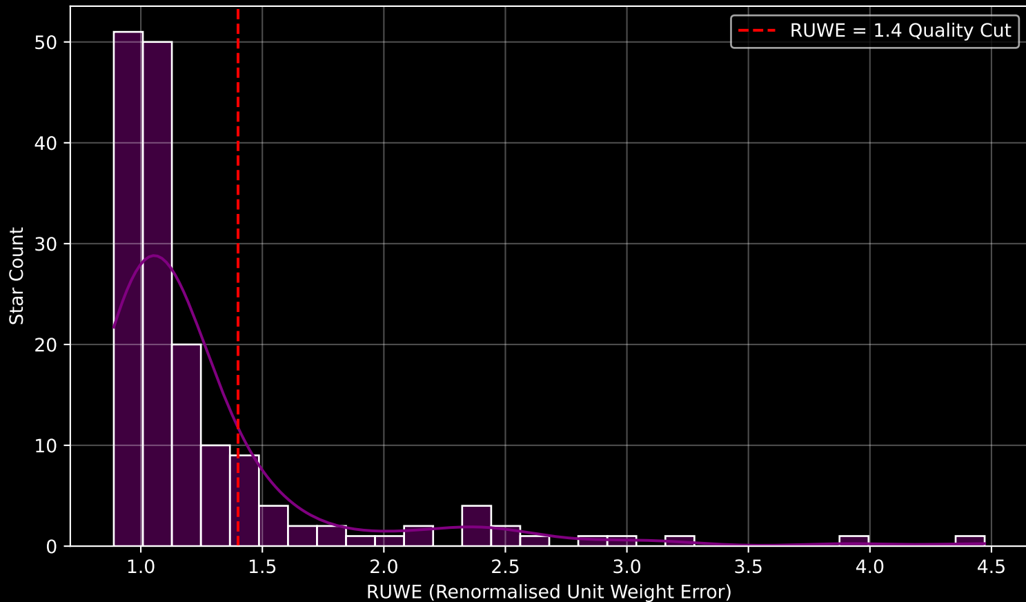
GAPOGEE DR17 Field [041+47_MGA] RUWE Distribution (n= 164)
