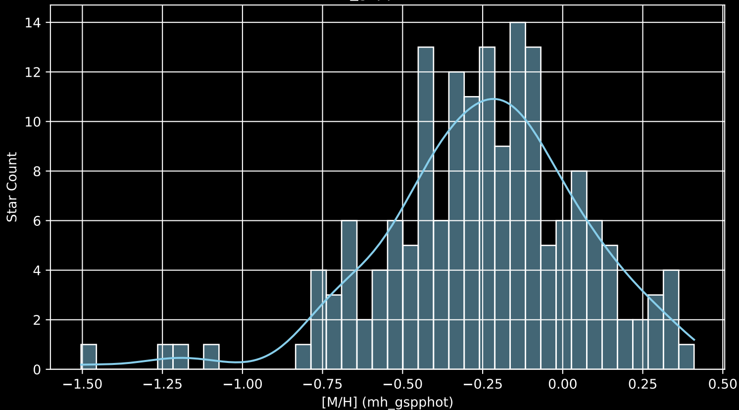
APOGEE DR17 Field: [041+47_MGA [M/H] (mh_gspphot) (n= 168)
